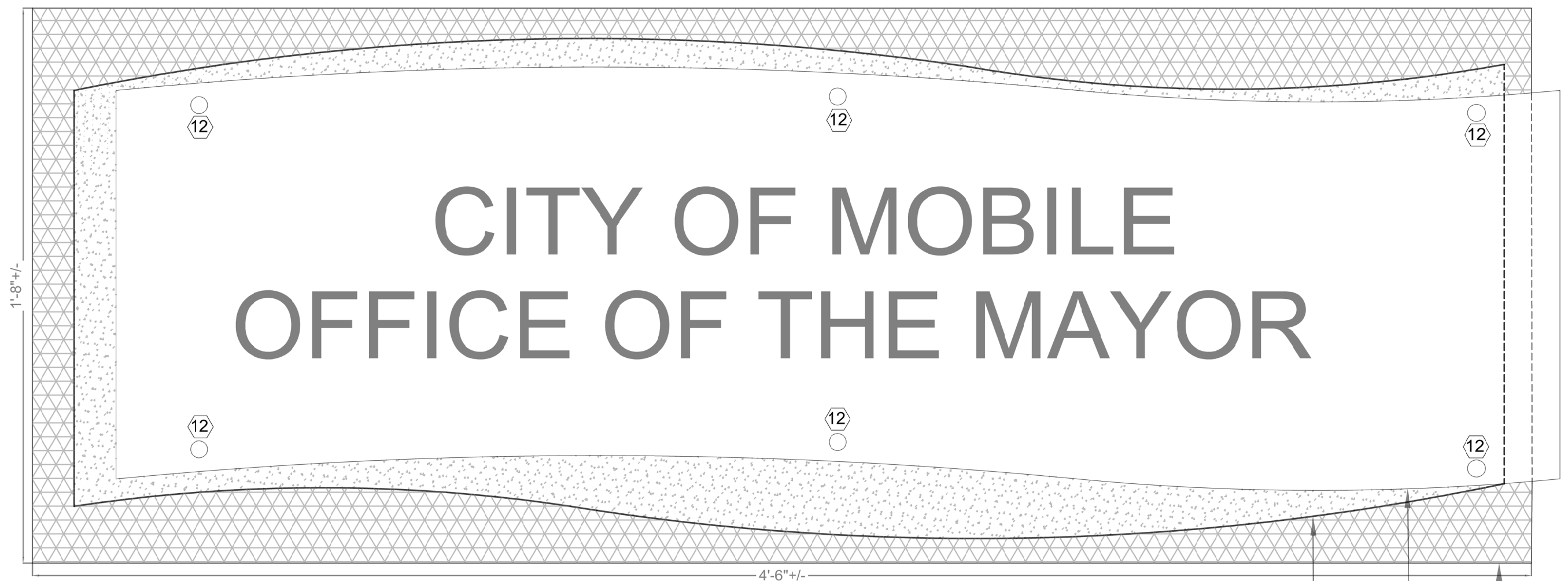
J SIGNAGE TYPE. SCALE 3" = 1'-0"
