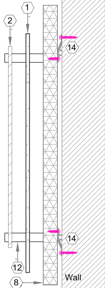
I SIGNAGE SIDE. SCALE 3" = 1'-0"
