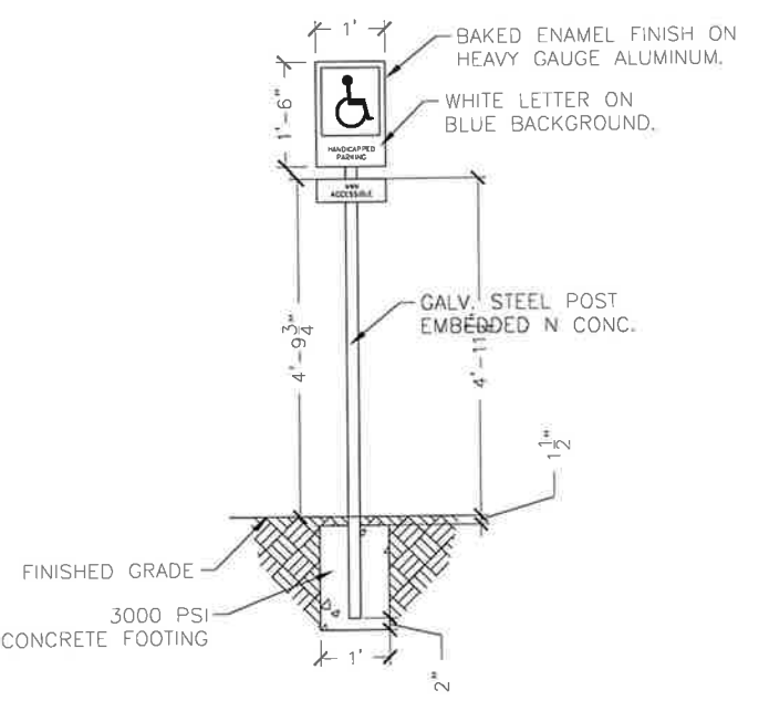
3 HC PARKING SIGN A-1 SCALE: 1/2" = 1'-0"
