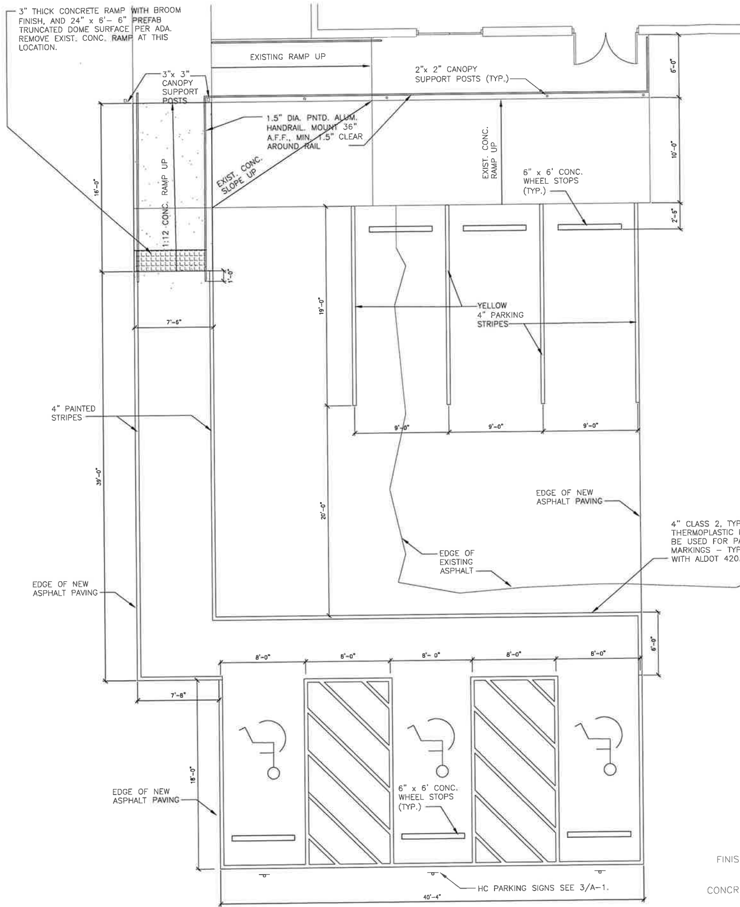
1 ACCESSIBLE PARKING PLAN SCALE: 1/4" = 1'-0"
