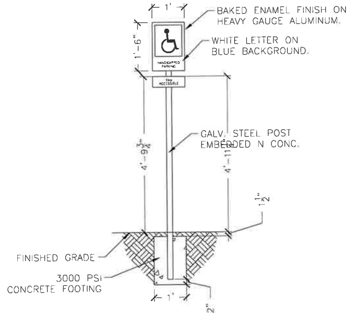
3 HC PARKING SIGN A-1 SCALE 1/2" = 1'-0"
