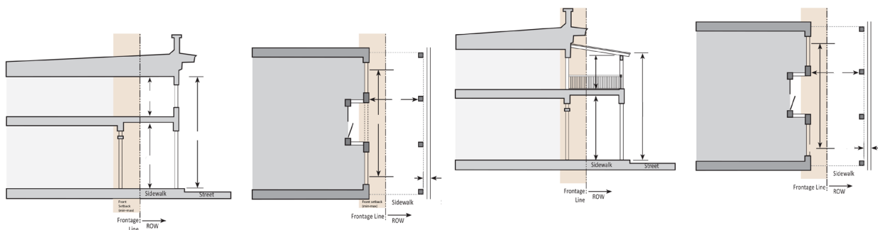
Figure 64-3-6.5 Arcade/Colonnade/Gallery Frontage Type
